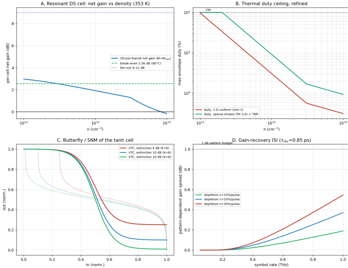
Figure 7. Pass 2, at 353 K unless noted. (A) DS single-transit net gain vs density, Eq. (2). (B) Thermal duty ceiling vs density, refined from Pass 1. (C) Static noise margins (butterfly construction) of the tanh cell at 6/10/20 dB extinction. (D) Pattern-dependent gain spread vs symbol rate at \tau = 0.85 ps.
