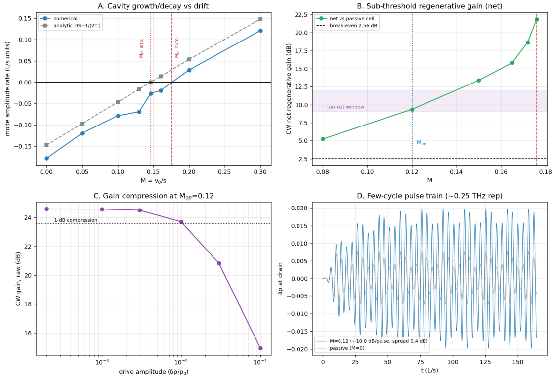
Figure 8. Pass 3, solver units ( M_{th,num} \approx 0.176 ; operating ratio M/M_{th} = 0.68 \approx 0.7 marked). (A) Cavity growth/decay rate vs drift, numerical vs analytic Eq. (2), both thresholds marked. (B) Sub-threshold CW regenerative net gain vs M ; break-even at the per-gate ( \lambda_p/2 ) loss, 2.56 dB in solver units; no-oscillation window shaded. (C) Gain compression vs drive amplitude at the working ratio — the logic rail. (D) The 0.25 THz few-cycle pulse train through the cell: +10 dB per pulse, 0.38 dB spread.
