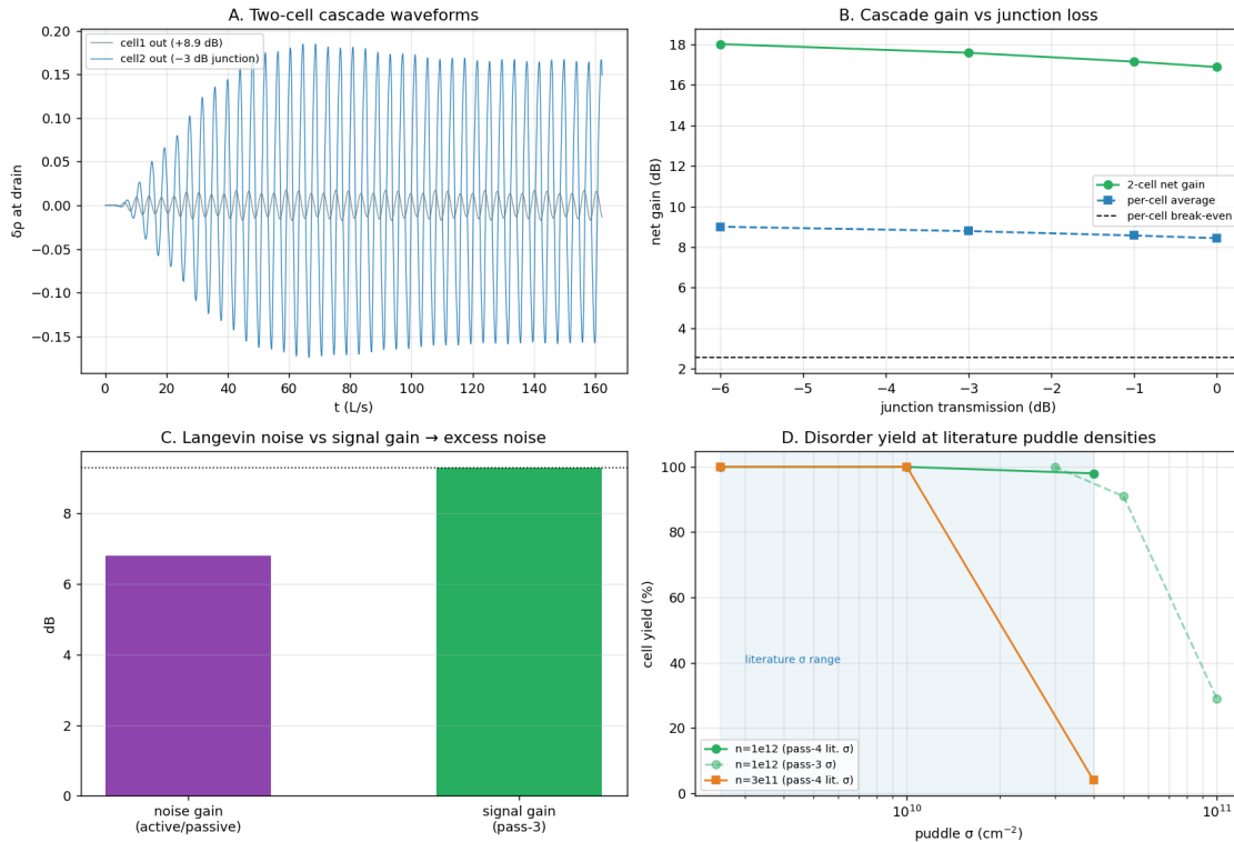
Figure 9. Pass 4. (A) Two-cell cascade waveforms through a -3 dB junction. (B) Net two-cell gain and per-cell average vs junction transmission. (C) Langevin noise-gain vs signal-gain comparison — preliminary: the added-noise bookkeeping in this panel awaits the explicit-convention re-derivation of Section 7.4. (D) Monte-Carlo cell yield vs puddle density \sigma , with the literature range shaded.
