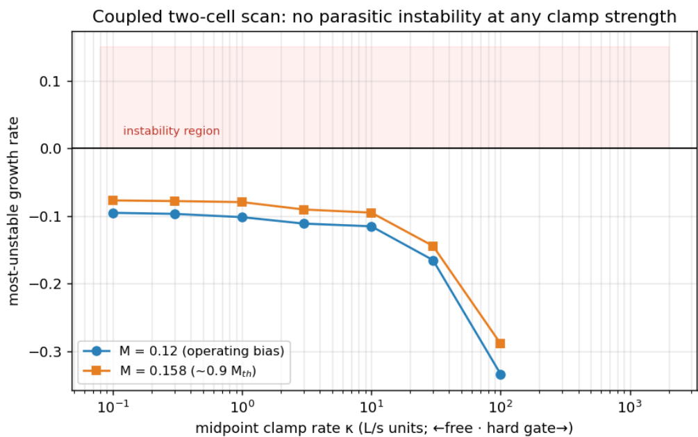
Figure 10. Pass 5: most-unstable growth rate of two coupled DS cells vs midpoint clamp strength, at the working bias and at 0.9\cdot M_{th} — no instability region is entered at any coupling.
