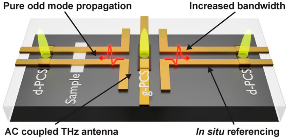
Figure 2. Monolithic launcher/detector/reference circuit, reproduced from Kusyak et al. [7] (CC BY 4.0): APL Photonics 10, 076117 (2025); generator switch (g-PCS) centered on a coplanar stripline with two symmetric detector switches (d-PCS) — galvanic isolation plus in-situ referencing. Used at the fabric edges for launch/read-out and reused mid-fabric as re-sync clock taps.
